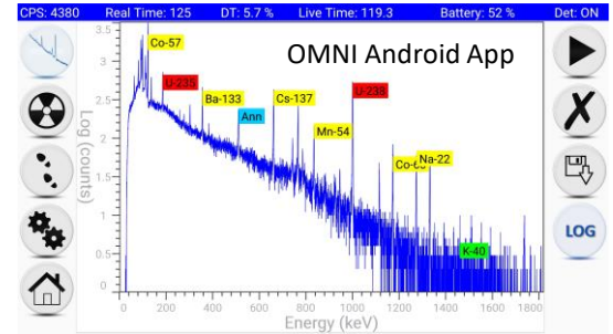
Spectroscopy
